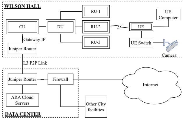
Figure 4: Skylark Deployment Architecture
