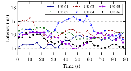
Figure 11: Latency from BS to UEs
