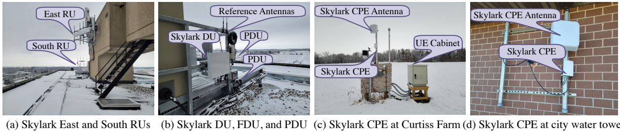
Figure 3: Field Deployment of Skylark Faros V2 System
