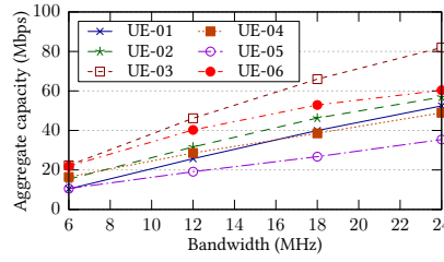
Figure 10: Capacity per UE
