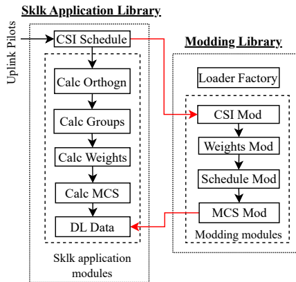
Figure 5: Modding API Architecture
