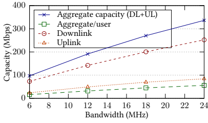
Figure 9: Capacity for 6 UEs
